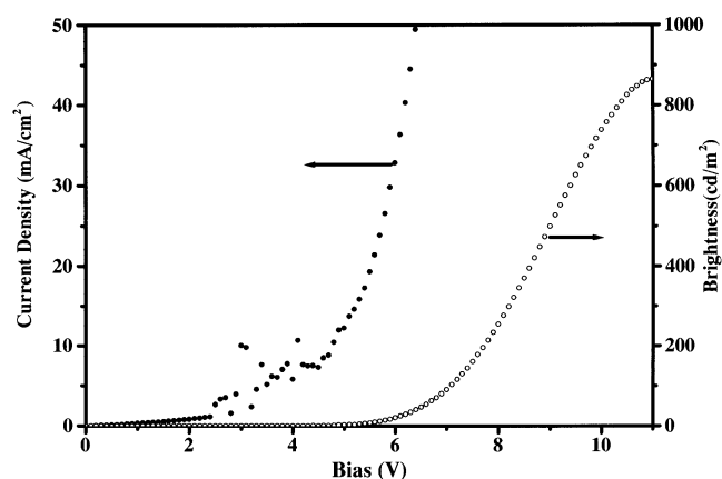
Figure 3. Current-voltage-luminescence ( I – V – L ) characteristics of the ITO/PEDOT/PFV/Al device.
